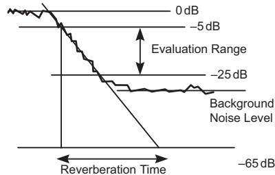
Fig. 1 Reverberation Decay Curve and Reverberation Time
