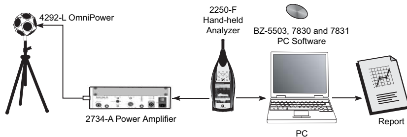
Fig. 5 Typical measurement setup using a loudspeaker source
