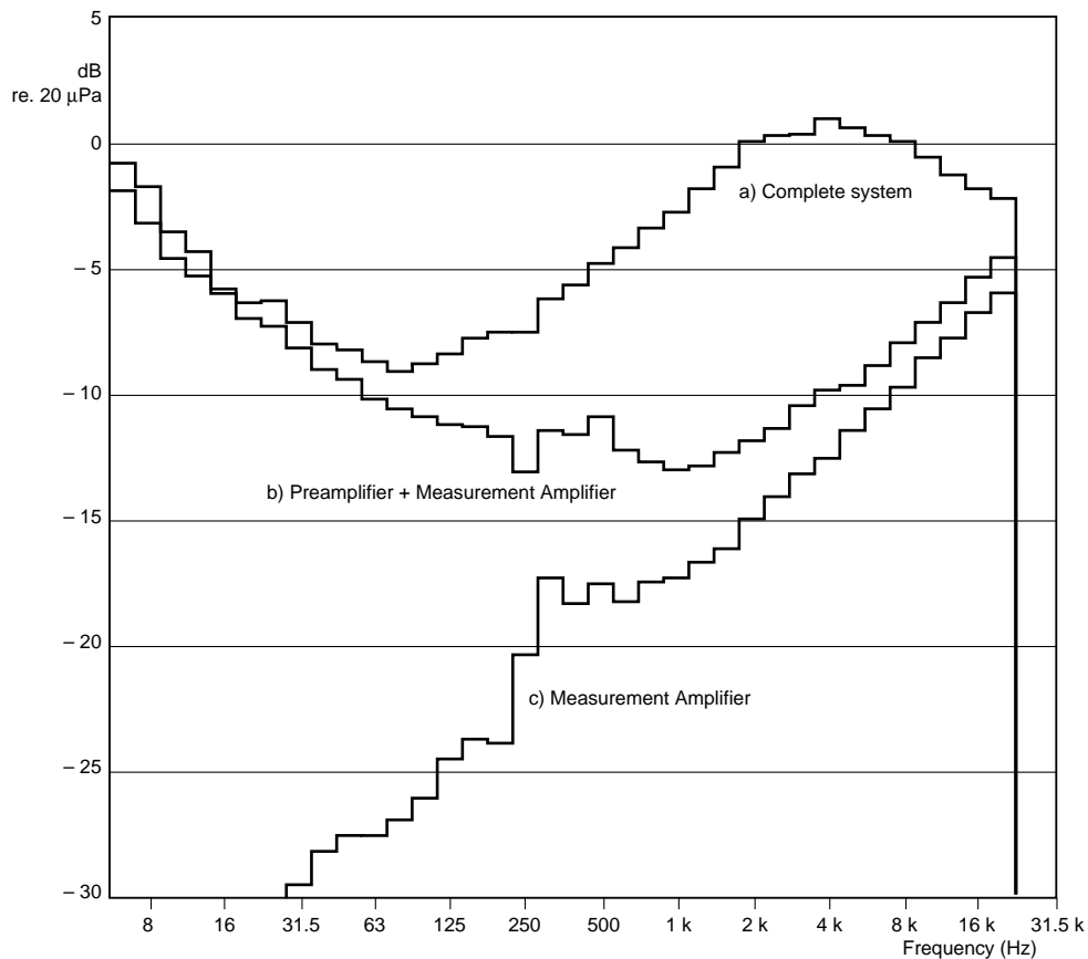
Fig.2.20 Equivalent levels of inherent noise (1/3 octave bandwidth) produced by the elements of a system equipped with a 1" free-field microphone (50 mV/Pa). The microphone, the preamplifier and the measurement amplifier are all significant noise sources in certain parts of the frequency range
