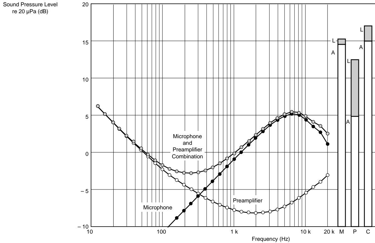
Fig. 2.21 Third Octave Noise Spectra of a system consisting of a free-field microphone ( 1/2'' , 50 mV/Pa) and a high quality preamplifier: The electrical preamplifier noise dominates at low frequencies while Brownian movements of the microphone diaphragm create the most significant noise at high frequencies. The columns to the right show Linear (20 Hz - 20 kHz) (L) and A-weighted (A) noise levels for the microphone (M), preamplifier (P) and combination (C)
