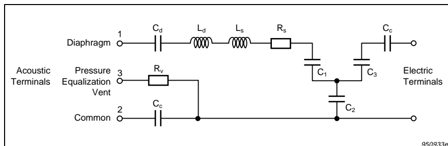
Fig. 2.13 Microphone model. The components of the equivalent electrical circuit represent stiffnesses, masses and damping of the electro-mechanical system. The response of the model depends on the exposure to sound pressure of the static pressure equalization vent (exposed: (3) connected to (1); unexposed: (3) to (2))
