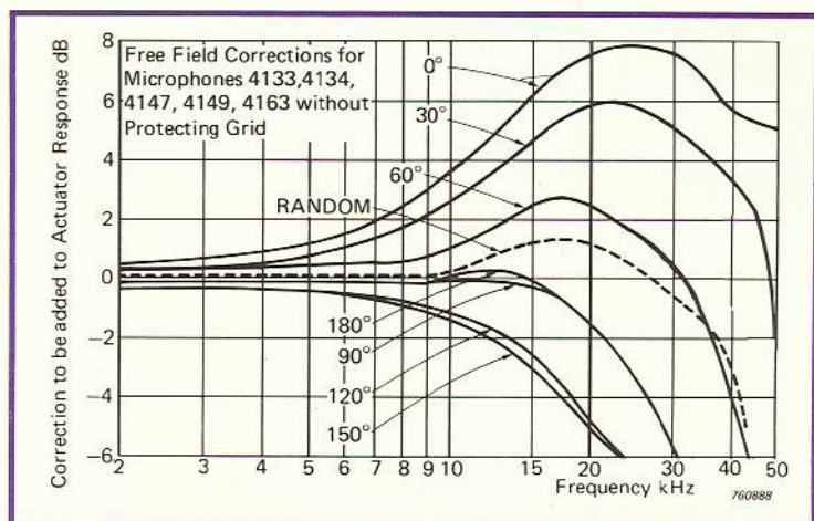
Example of free-field correction curves
