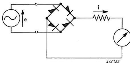
Fig. 17. Schematic diagram of Average rectifier.
