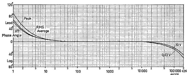
Fig. 14. Typical phase-frequency response for the Electronic Voltmeter Type 2409/2416. At low frequencies the phase shift is somewhat dependent upon the METER SWITCH setting, and at high frequencies, upon METER RANGE.
