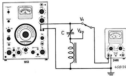
Fig. 9. Measurement of quality-factor of inductances.
