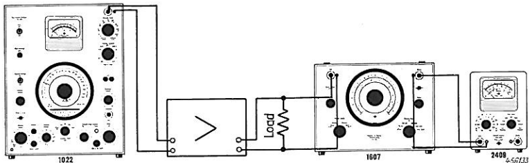
Fig. 8. Measuring arrangement for distortion measurements.
