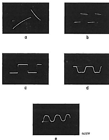
Fig. 15. Oscilloscope photographs of the waveform at the output jack when a square wave is applied to the amplifier input.
