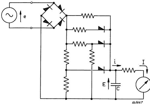
Fig. 20. Schematic diagram of the RMS rectifier circuit having characteristics of the type shown in Fig. 21.
