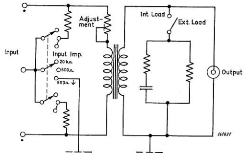
Fig. 11. The B & K Input Transformer TI 0001.
